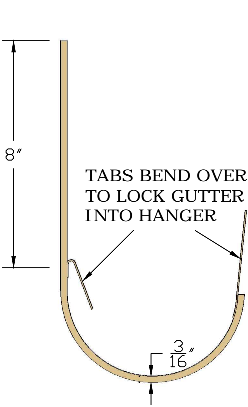
SIDE VIEW
