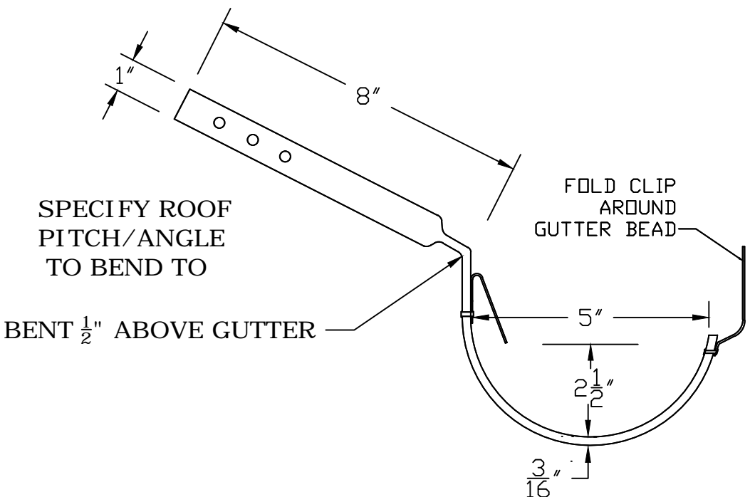
SIDE VIEW
